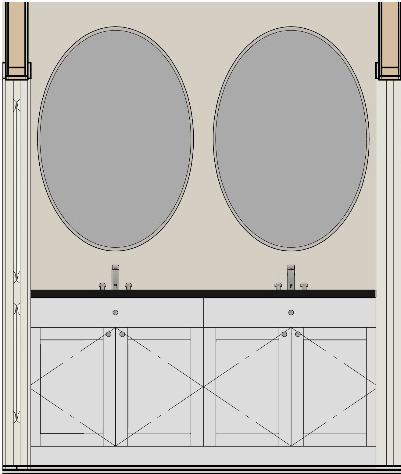
E9 Elevation 4 1 in = 1 ft
