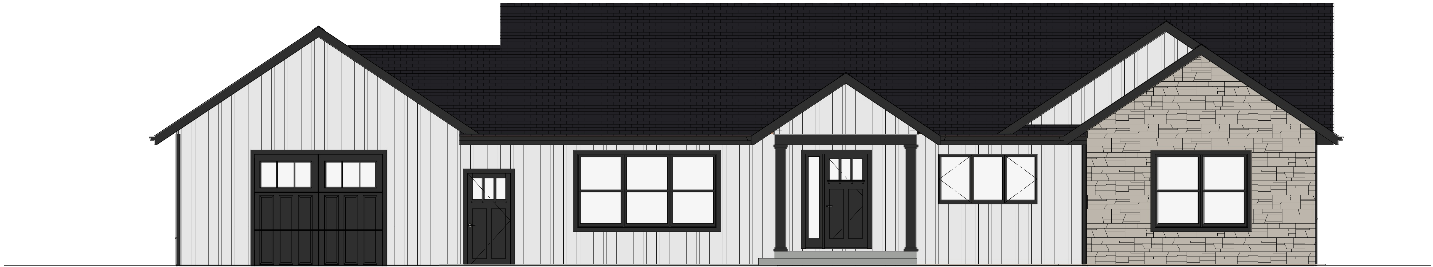
E2 Exterior Elevation Front 1/4 in = 1 ft
